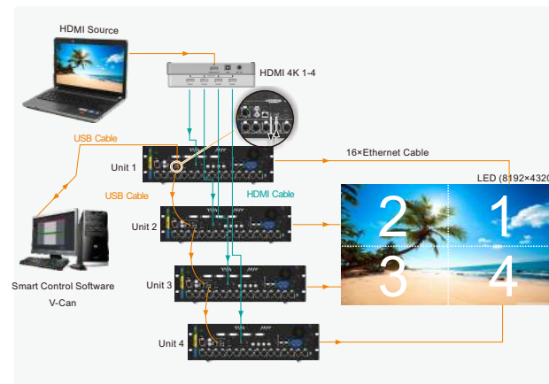
4 NovaPro UHD Jr units for image mosaic
