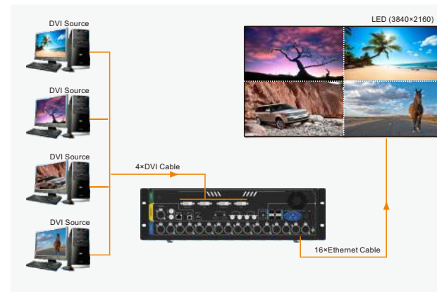
DVI MOSAIC - 4 x input source: 1920x1080@60Hz
