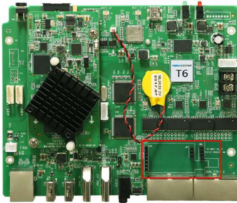
Figure 3-3 Installation position
